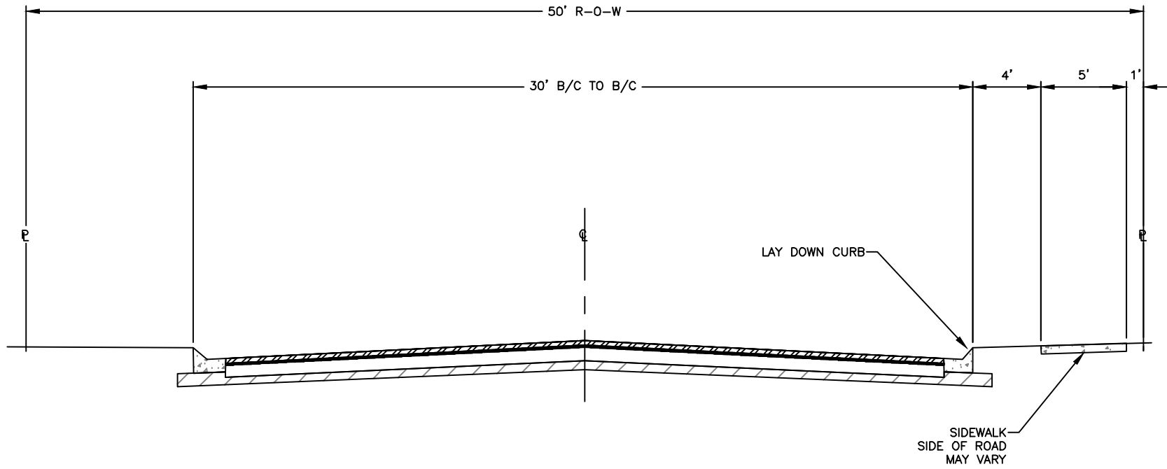
TYPICAL LOCAL STREET CROSS SECTION N.T.S.
